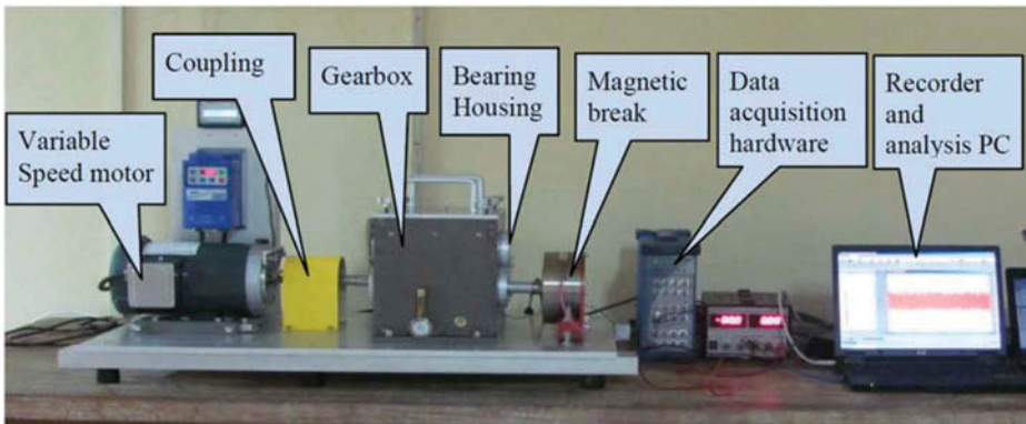
Figure 5. Experimental setup.
