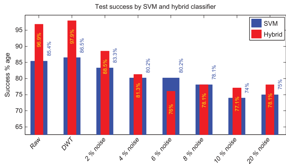
Figure 13. Comparative performance of SVM and hybrid classifier.
